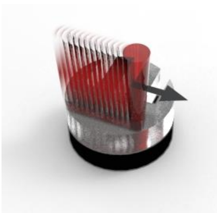
Figure: Principle of quasi-simultaneous welding
