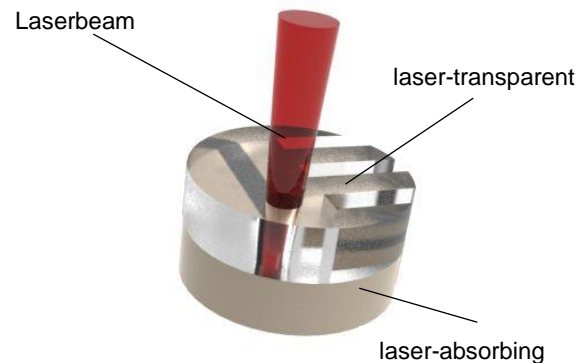
Figure: Principle of laser transmission welding
