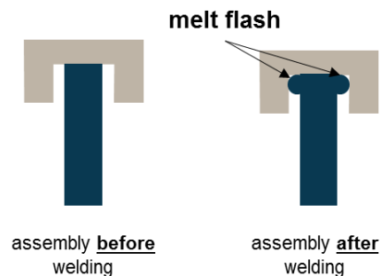
Figure: Melt flash cover
