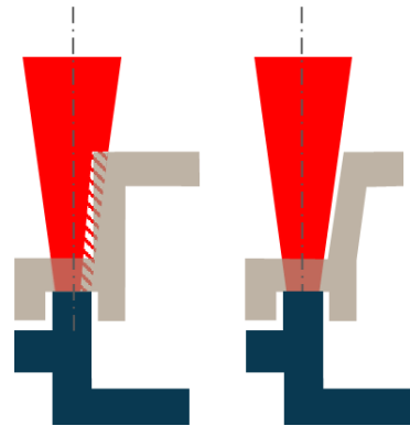
Figure: Beam shadow of laser beam
